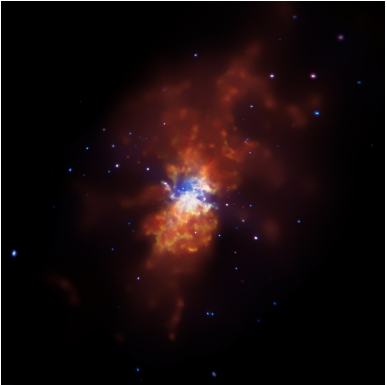
Galactic Wind (Provided)
